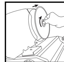
BLADE REMOVAL
